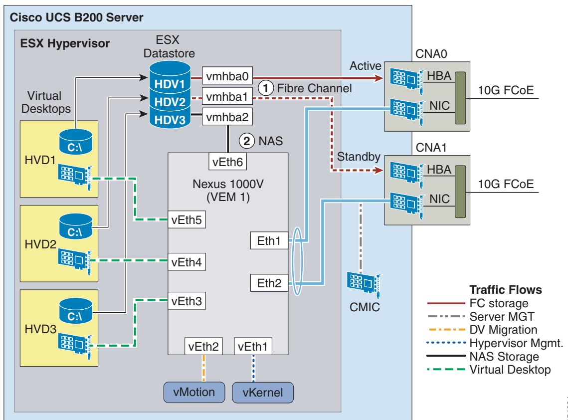
Figure 17 Data Center Connectivity (vSphere Example)
