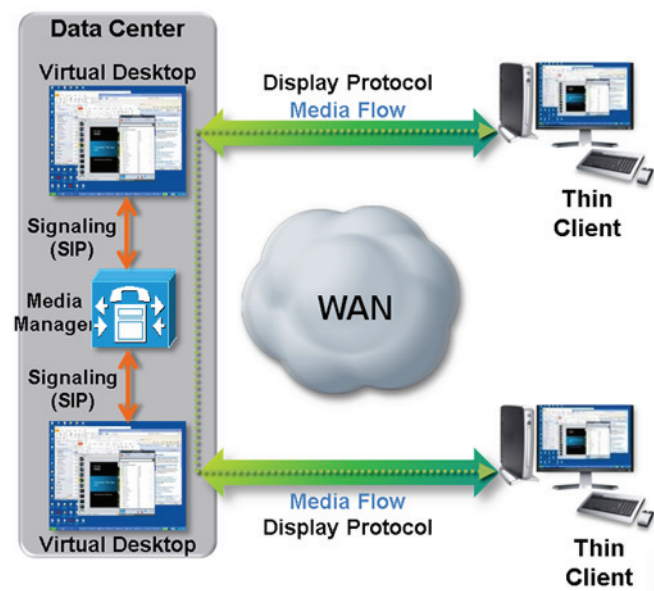
Figure 36 IP Telephony in traditional Virtual Desktops
