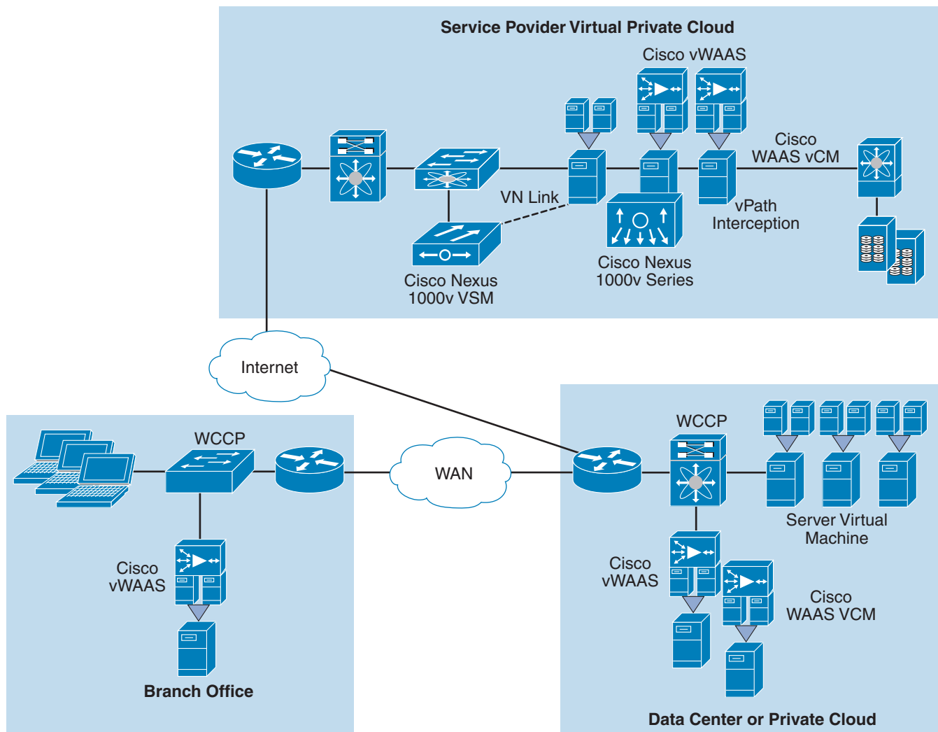
Figure 25 Cisco vWAAS
